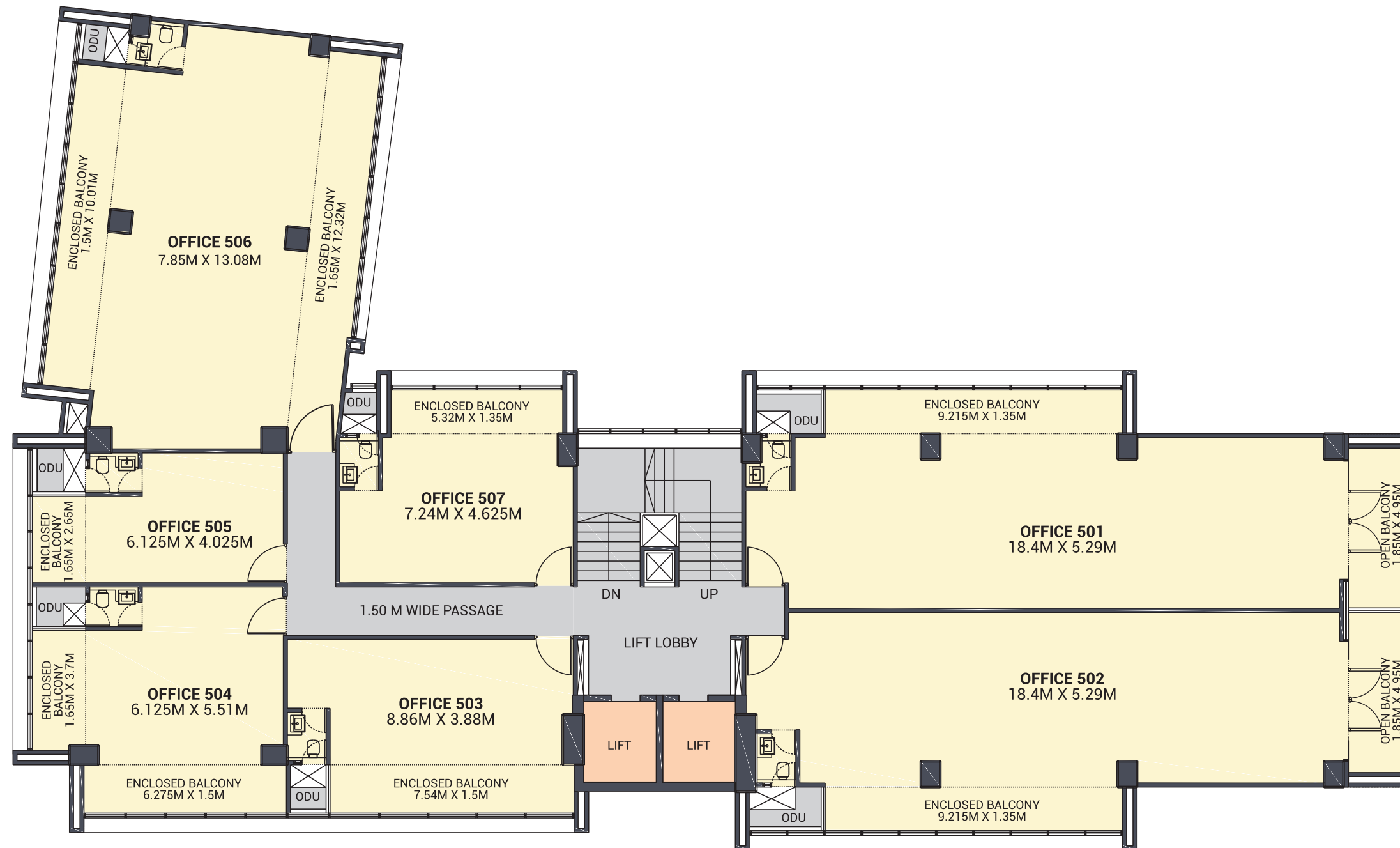
FIFTH FLOOR PLAN - OFFICES
