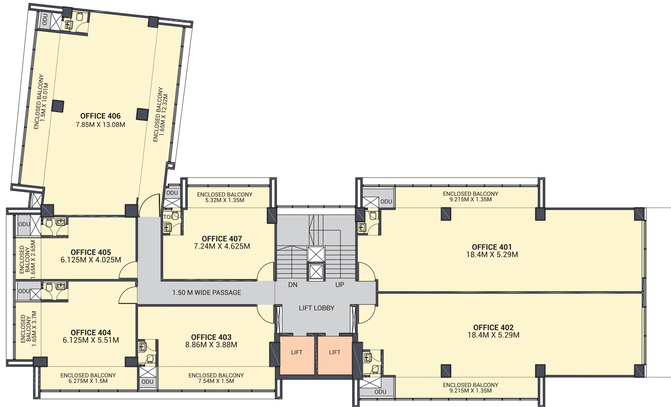
FOURTH FLOOR PLAN - OFFICES
